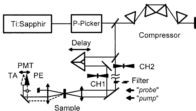
FIGURE 1 Schematic representation of the experimental setup for the 2PE and TA measurements. Ti:Sapphire, laser; P-Picker, pulse picker; CH1 and CH2, mechanical choppers; PMT, photomultiplier; TA and PE, locations of the PMT by transient absorption and photon echo measurements, respectively.
